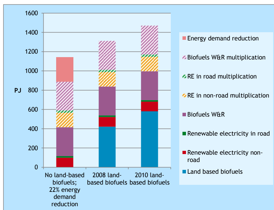
Figure 19 Scenario 1: Contribution of the various options, in PJ
