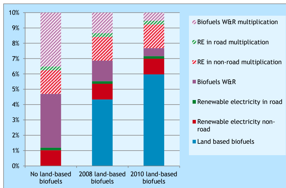
Figure 22 Scenario 2: Renewable energy mix to meet the 10% RED target
