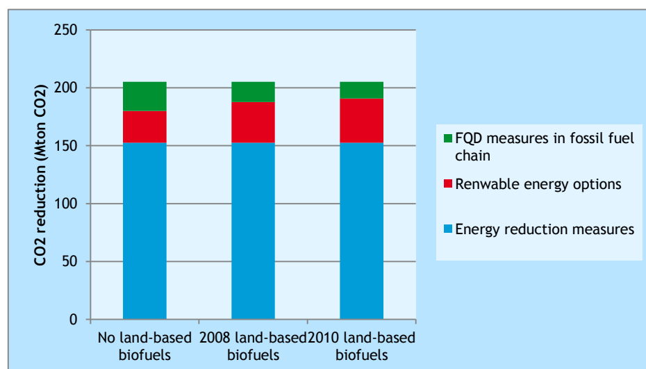
Figure 25 Scenario 2: Total CO 2 reduction achieved (Mton)
