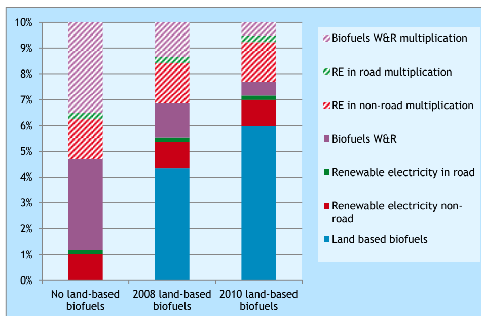
Figure 1 Scenario 2: Renewable energy mix to meet the 10% RED target
