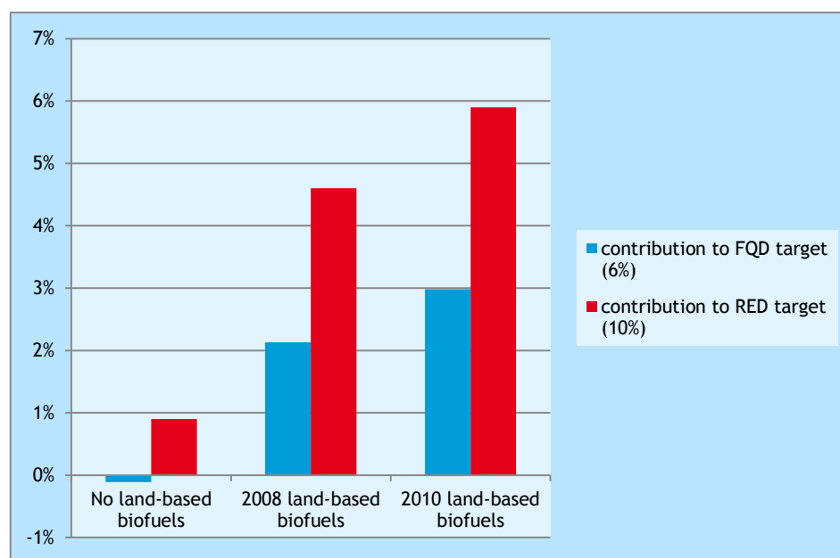
Figure 11 Contribution of the different assumptions to the RED and FQD targets
