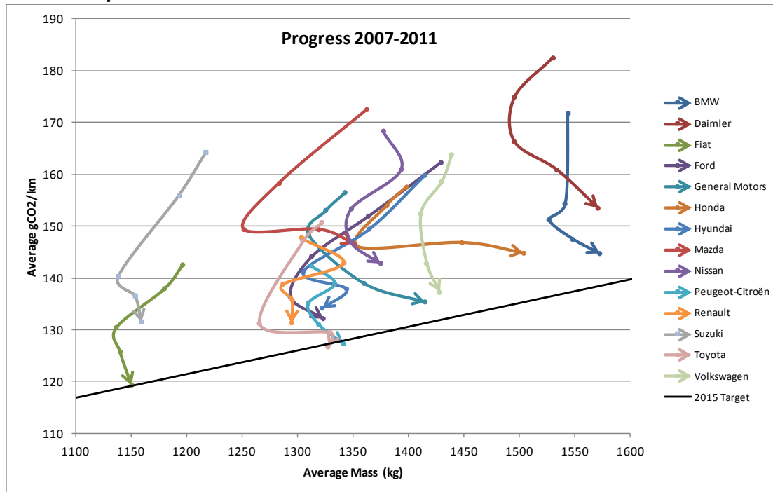
Graph 5: development in fleet-average weight and CO 2 per carmaker over the 2007-2011 period
