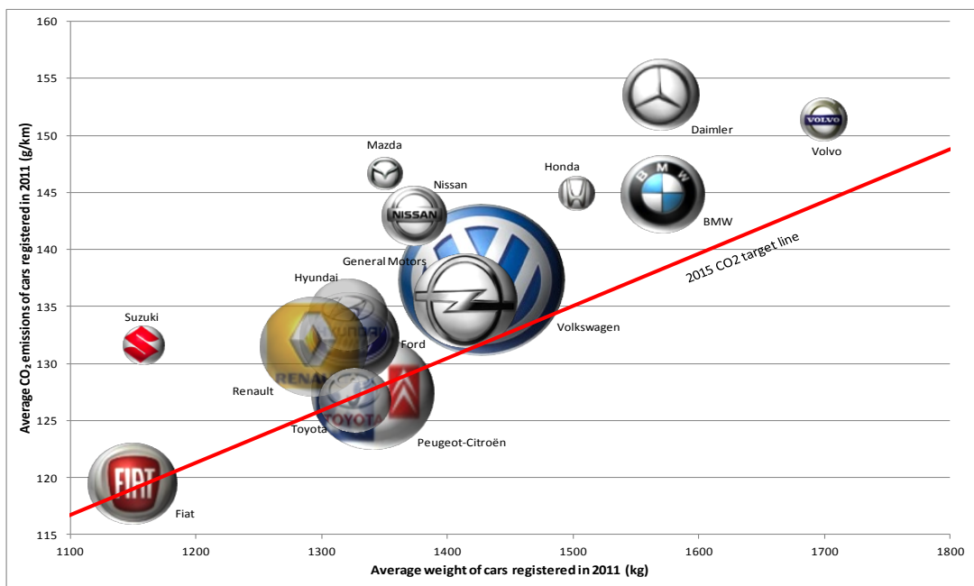
Graph 4: fleet-average weight and fleet-average CO 2 emissions by carmaker, compared with EU target line
