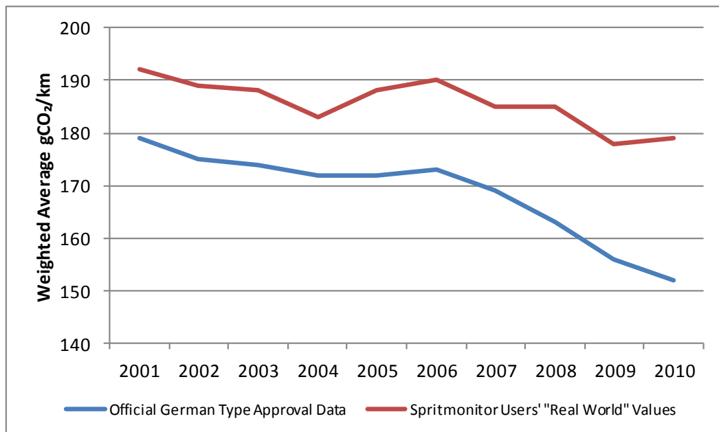
Graph 3: CO 2 emissions according to official German type-approval data and real-world values
