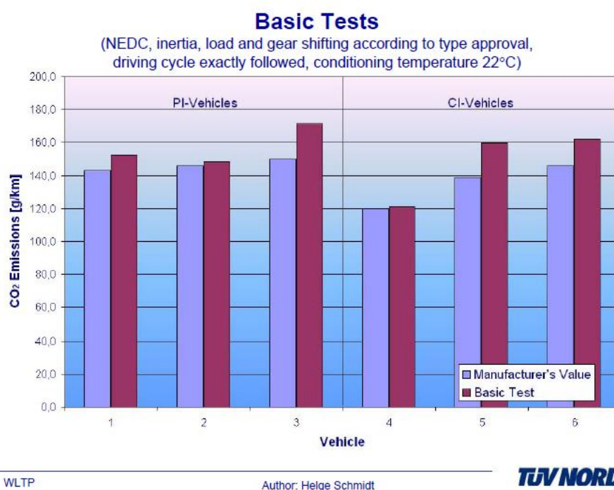
Figure A2.2: Comparison of manufacturers’ CO 2 results with Schmidt and Johannsen’s own tests
