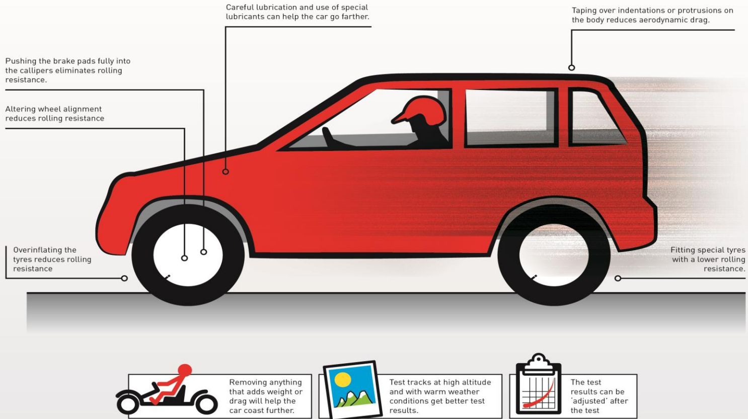
Figure 7: Specific manipulations of the road load test
